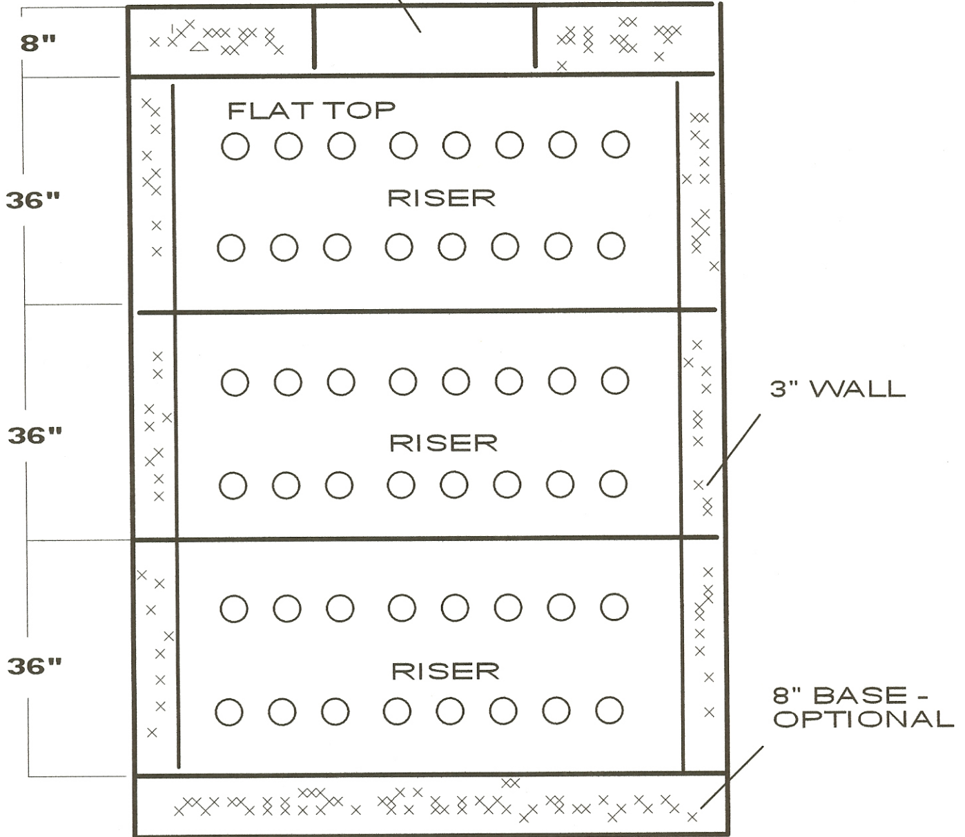
Section View of Dry Well
