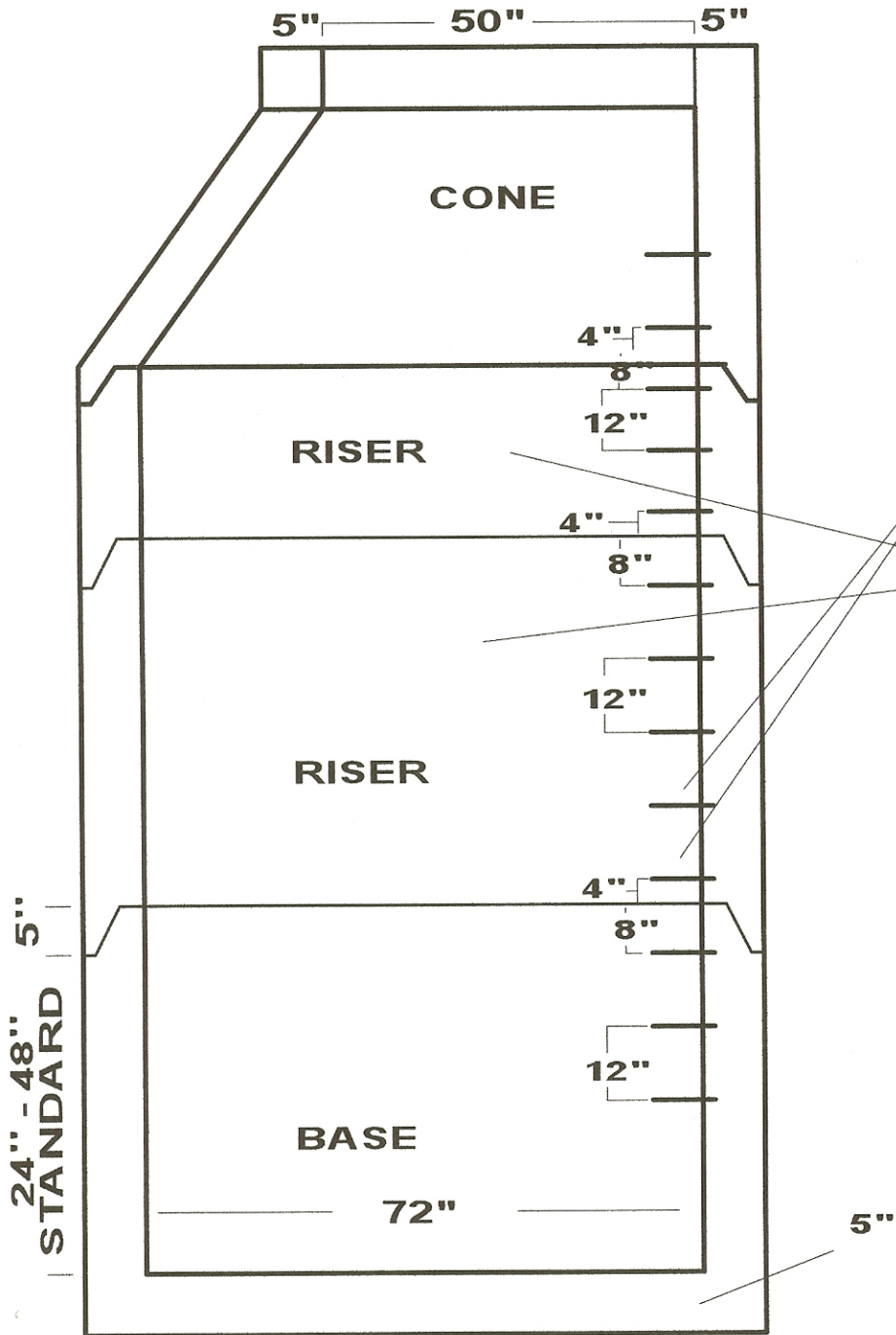
SECTION VIEW OF CONE MANHOLE
