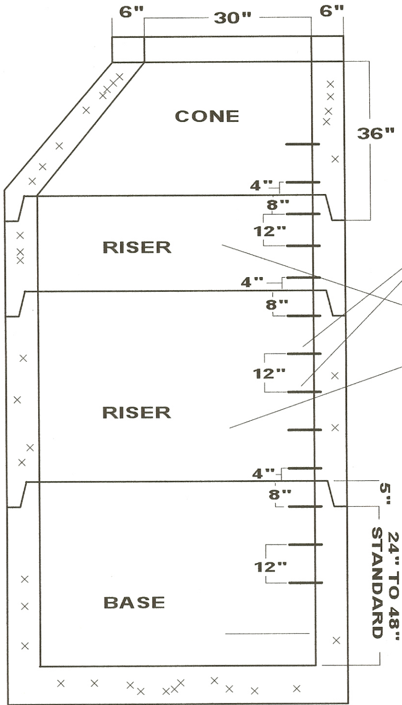
SECTION VIEW OF CONE MANHOLE
