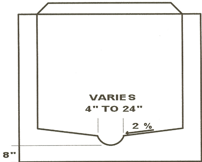
INVERT CROSS SECTION
