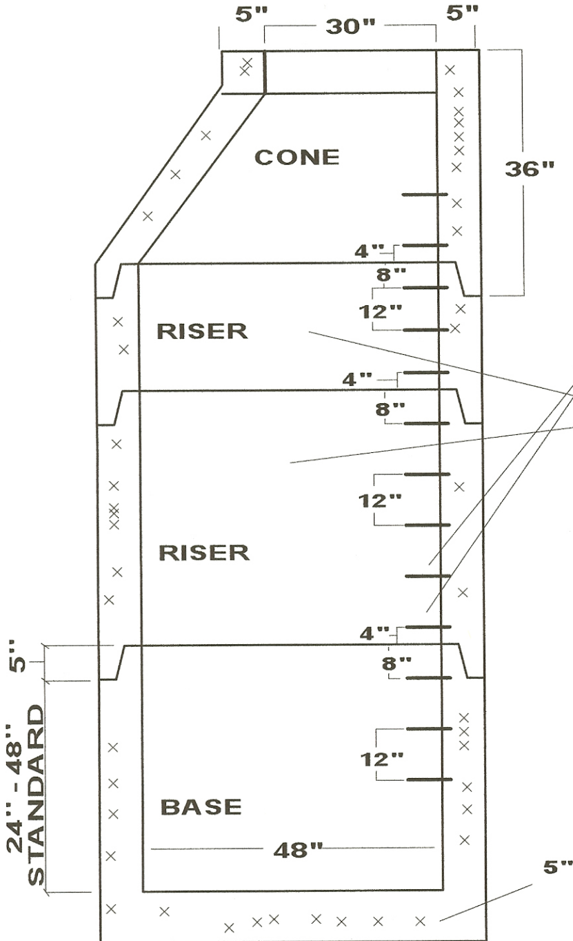
SECTION VIEW OF CONE MANHOLE
