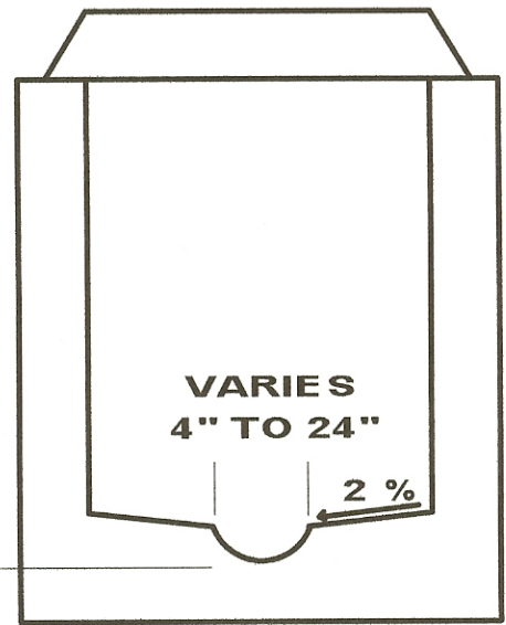
INVERT CROSS SECTION
